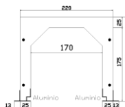
C2220
